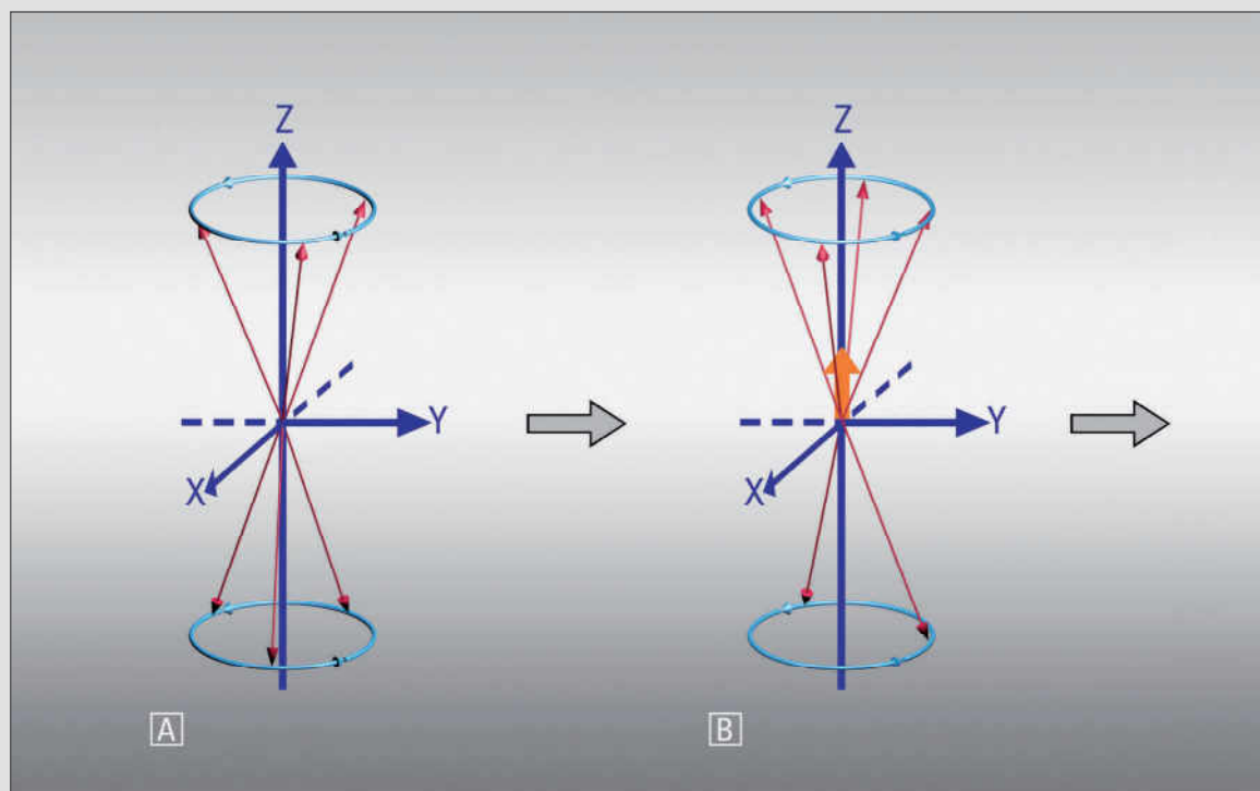
Fig. 17: After the RF pulse is switched off, protons go back from their higher to the lower state of energy, i.e. point up again. This is illustrated “one-by-one”. The effect is that longitudinal magnetization increases and grows back to its original value. Note that for simplicity the protons were not depicted as being in phase: this subject is covered in more detail in figures 20 and 26.
