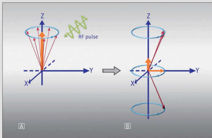
Fig. 13: The radio wave has two effects on the protons: it lifts some protons to a higher level of energy (they point down), and it also causes the protons to precess in step, in phase. The former results in decreasing the magnetization along the z-axis, the so-called longitudinal magnetization. The latter establishes a new magnetization in the x-y-plane ( \rightarrow ), a new transversal magnetization, which moves around with the precessing protons.
